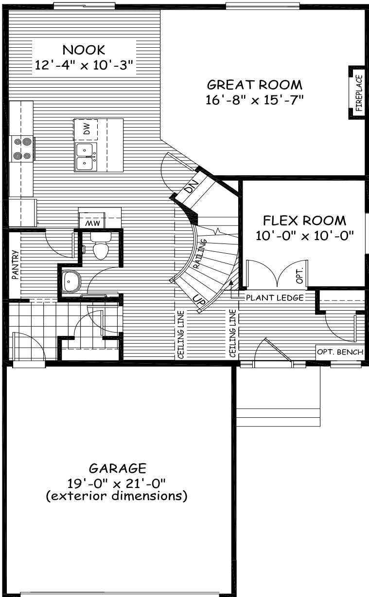
Main Floor 1020 sqft
