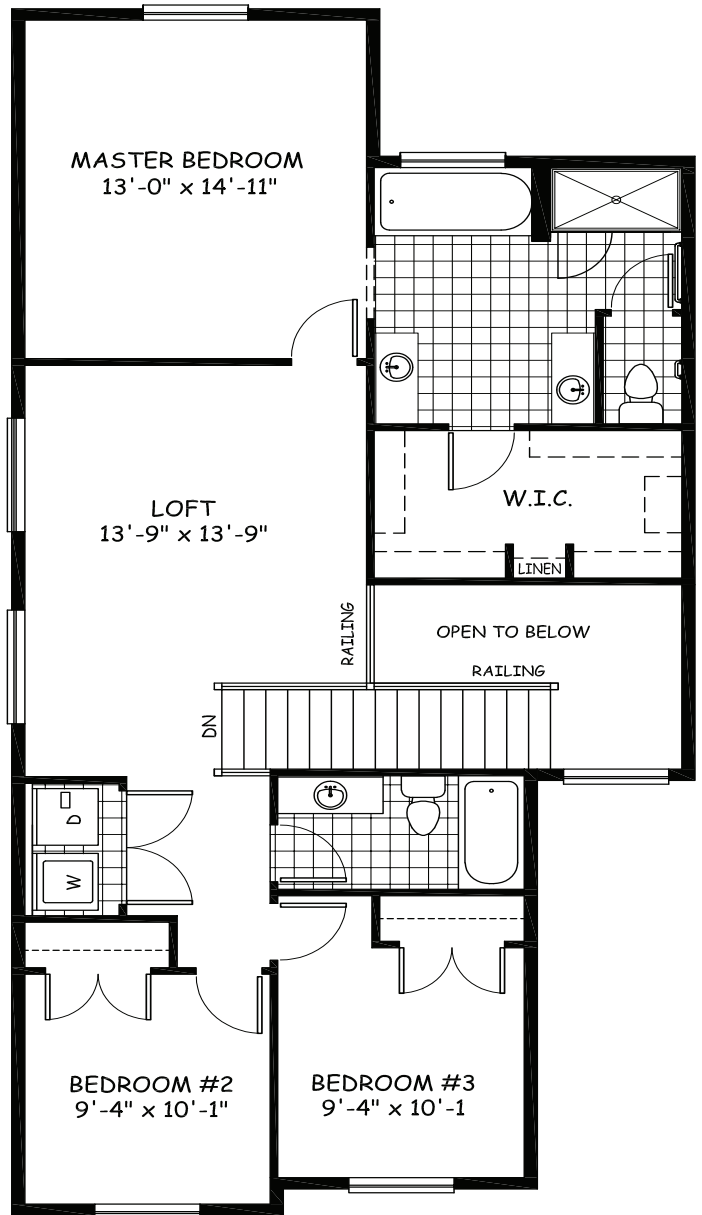
Upper Floor 1063 sqft
