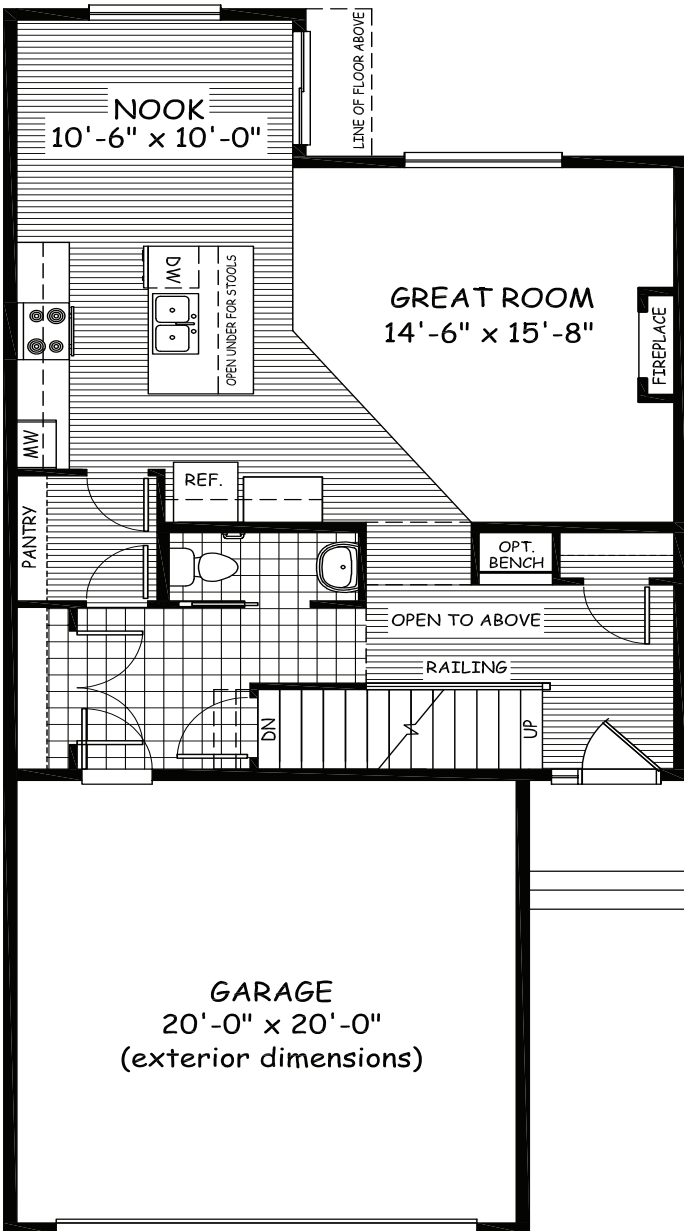
Main Floor 790 sqft
