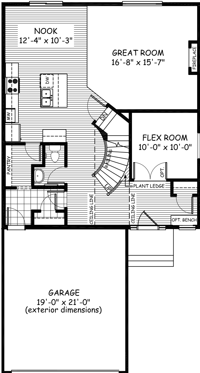
Main Floor 1020 sqft
