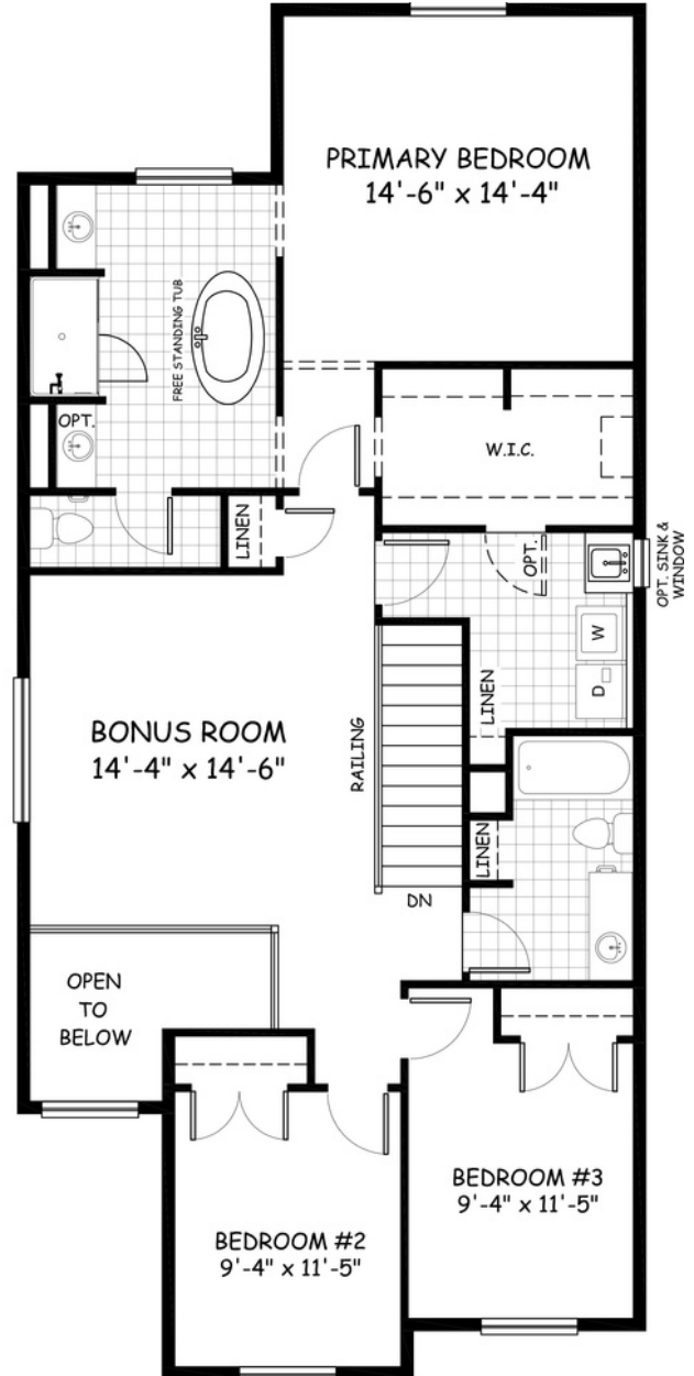
UPPER 1230 sq.ft.
