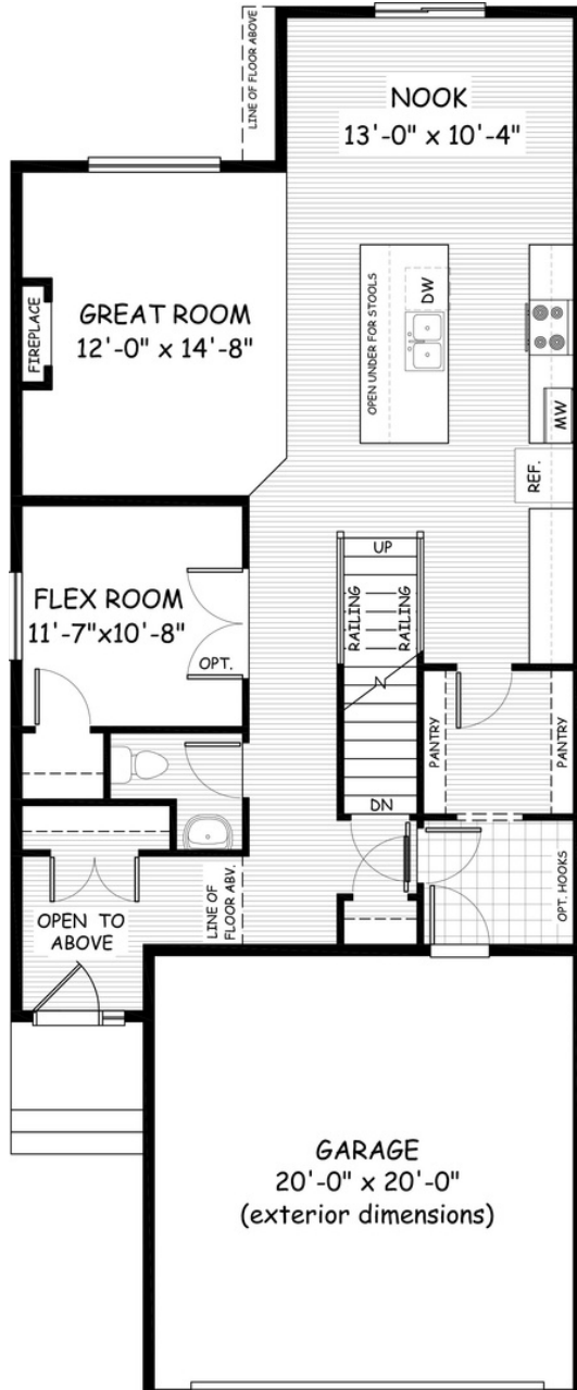
MAIN 1053 sq.ft.
