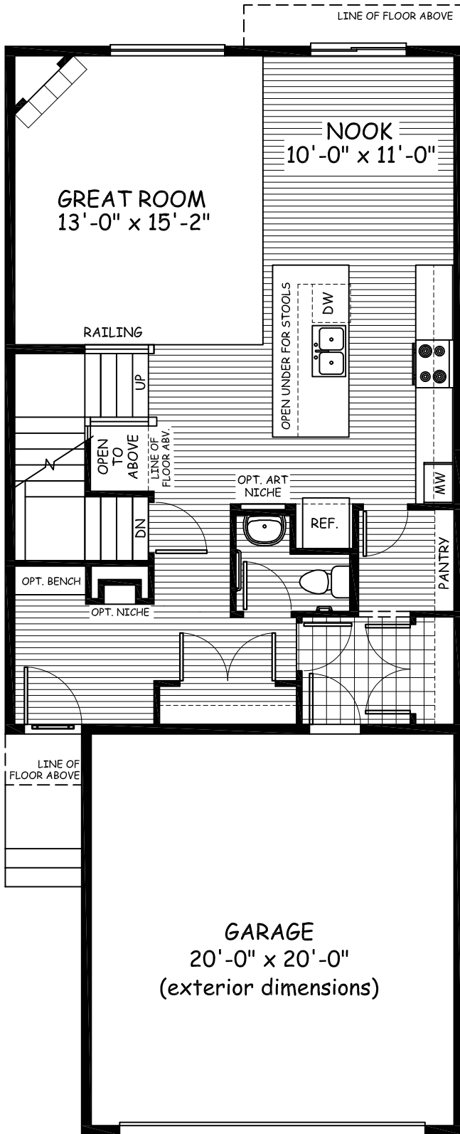
Main Floor 865 sqft
