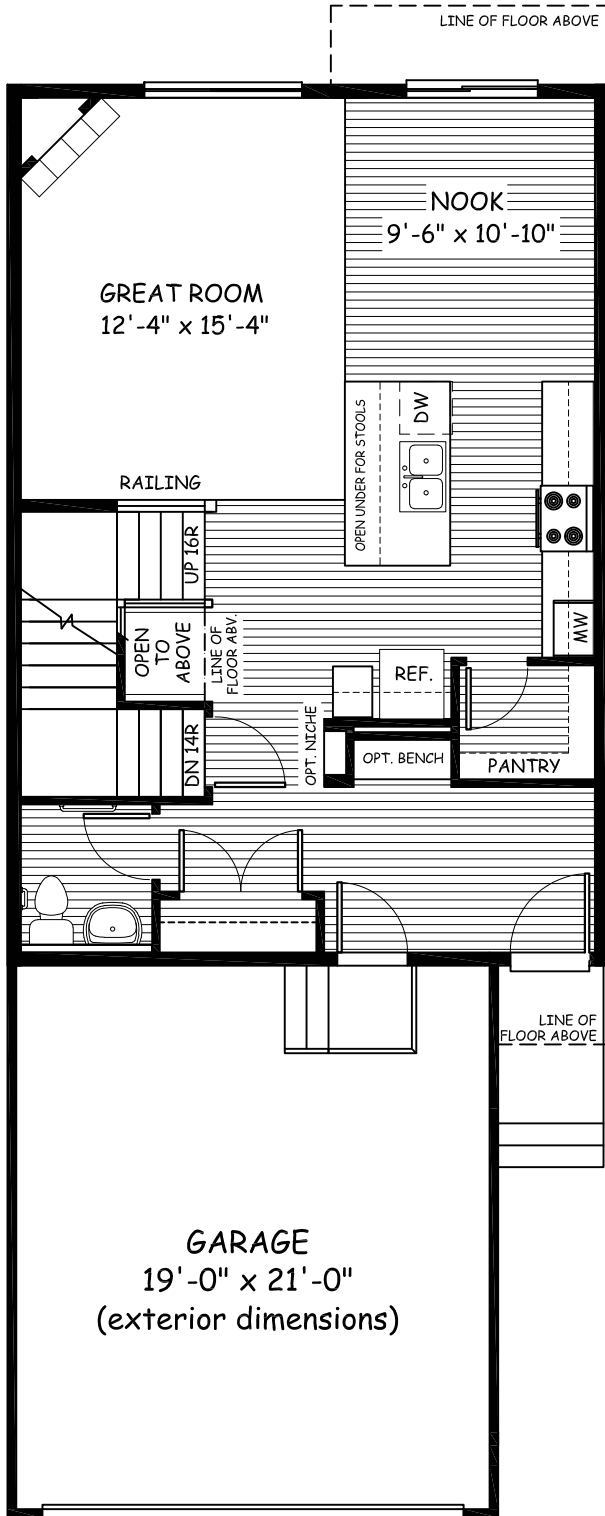
Main Floor 770 sq. ft.
