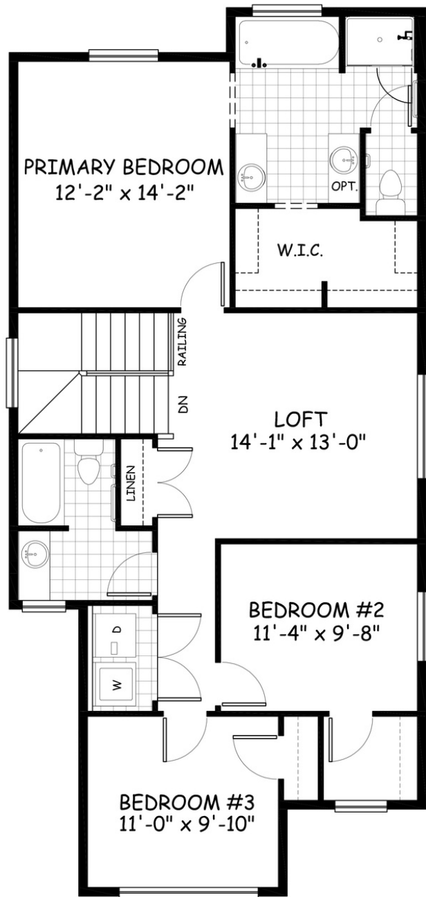
UPPER 1027 sq.ft.
