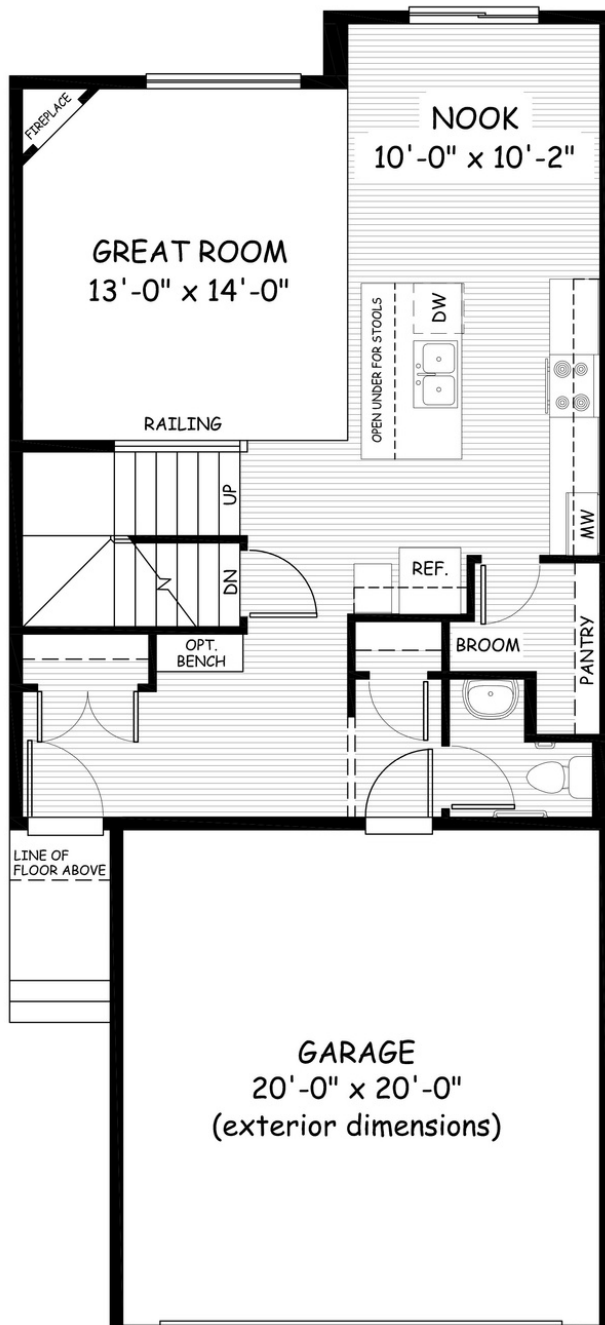
MAIN 750 sq.ft.
