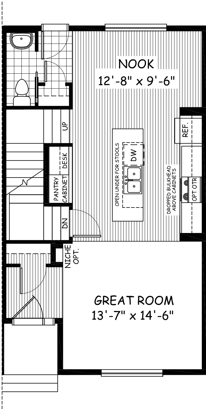
Main Floor 653 sqft
