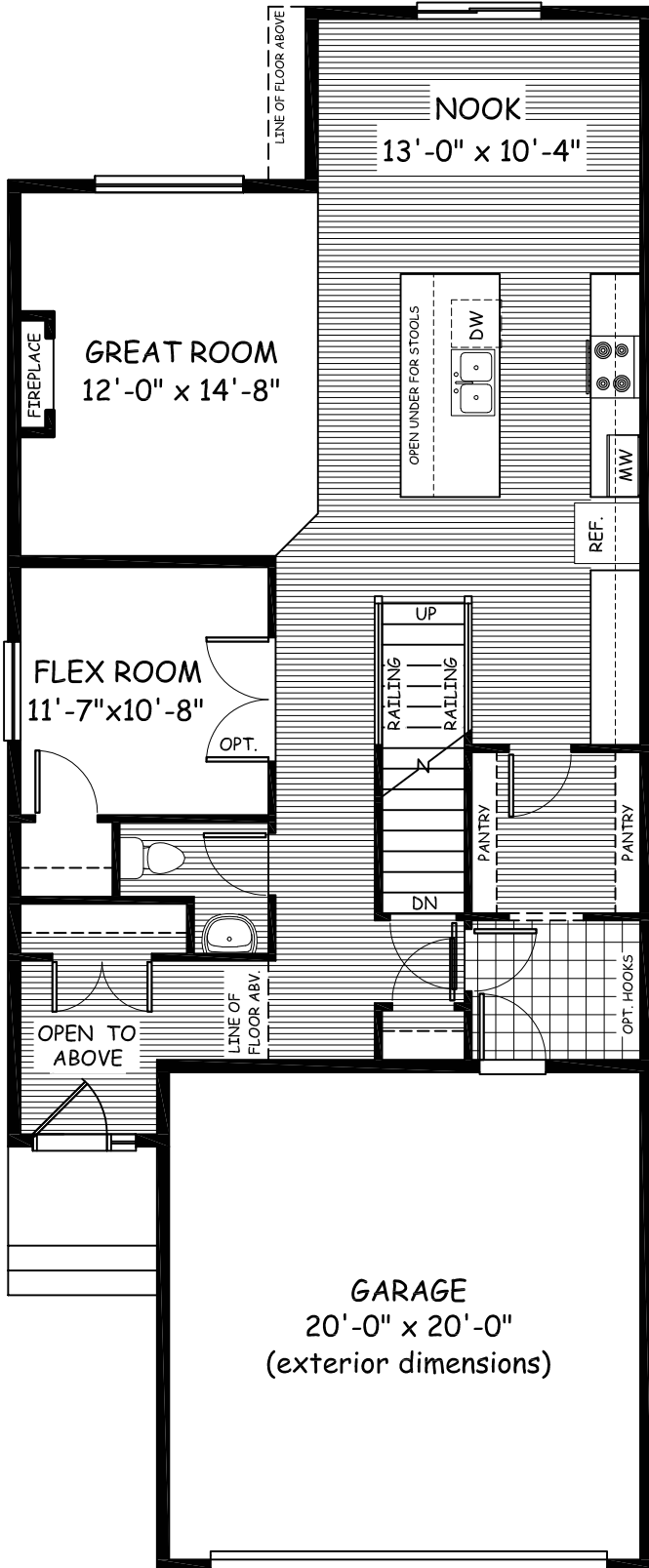
Main Floor 1053 sqft
