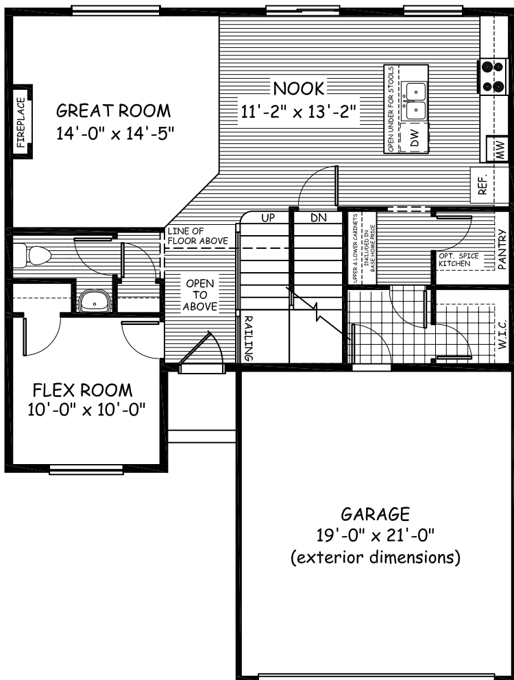
Main Floor 927 sq. ft.
