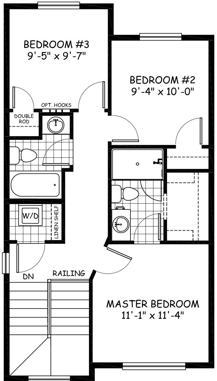
Upper Floor 609 sqft
