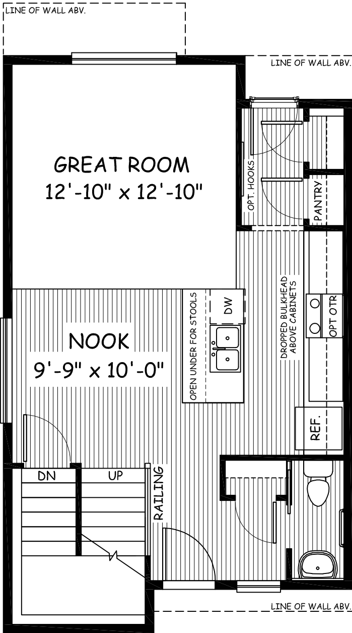
Main Floor 616 sqft
