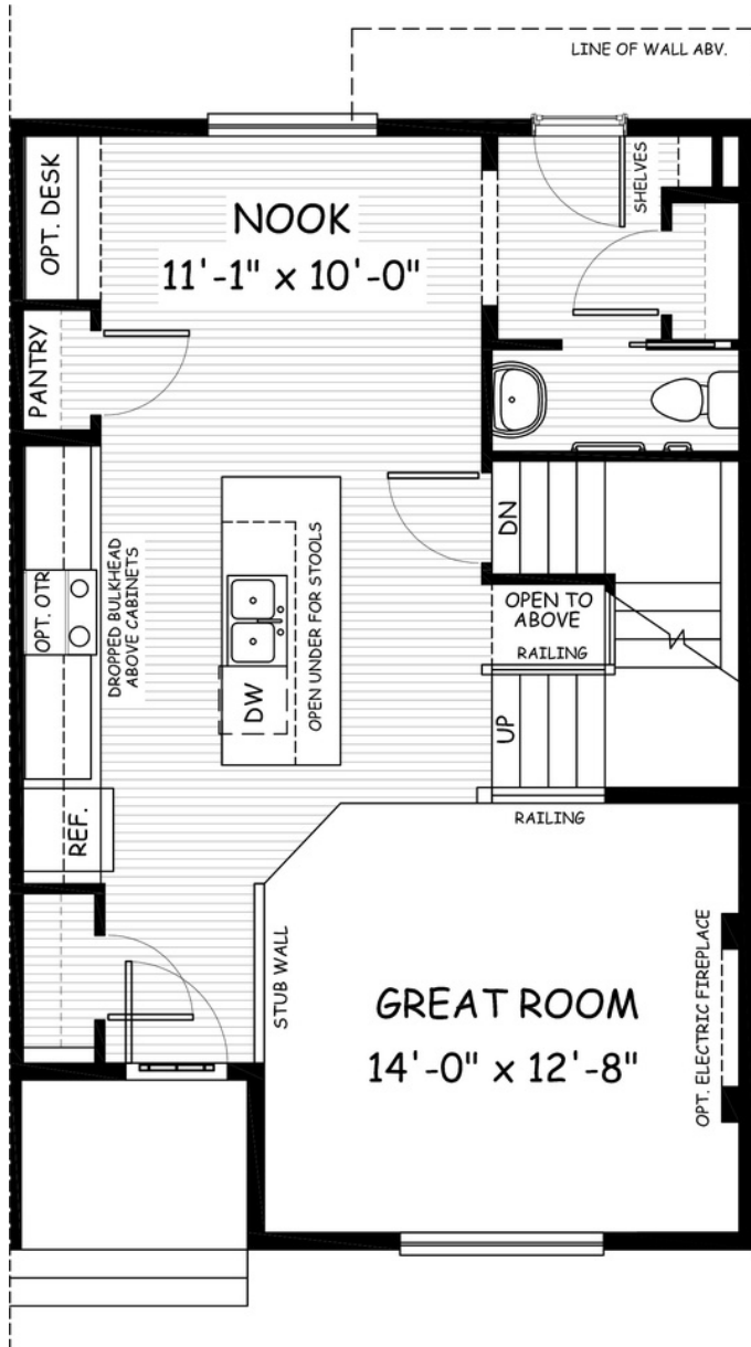
MAIN 698 sq.ft.
