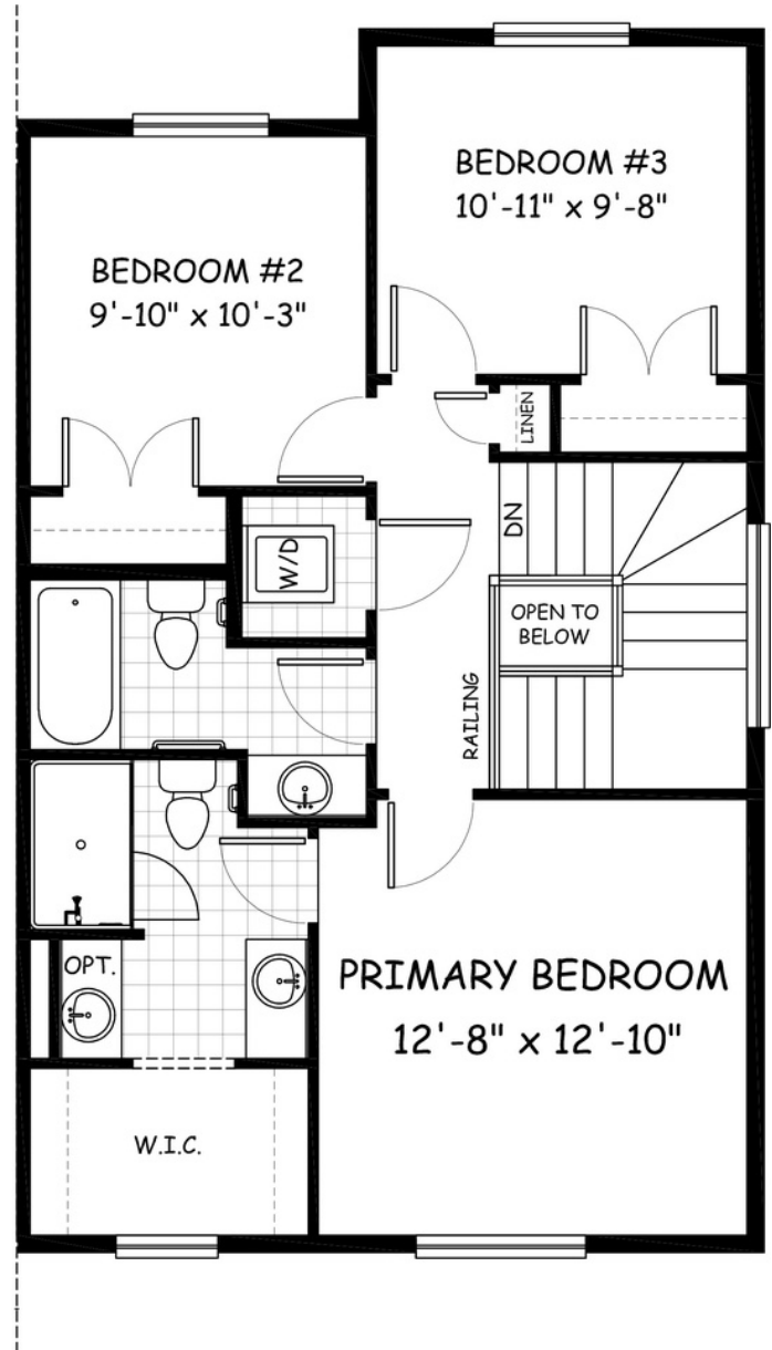
UPPER 695 sq.ft.
