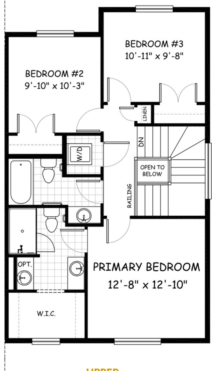
UPPER 695 sq.ft.
