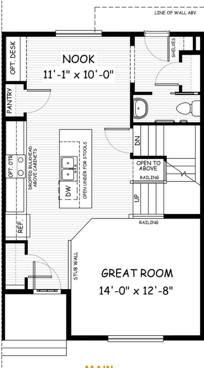
MAIN 698 sq.ft.
