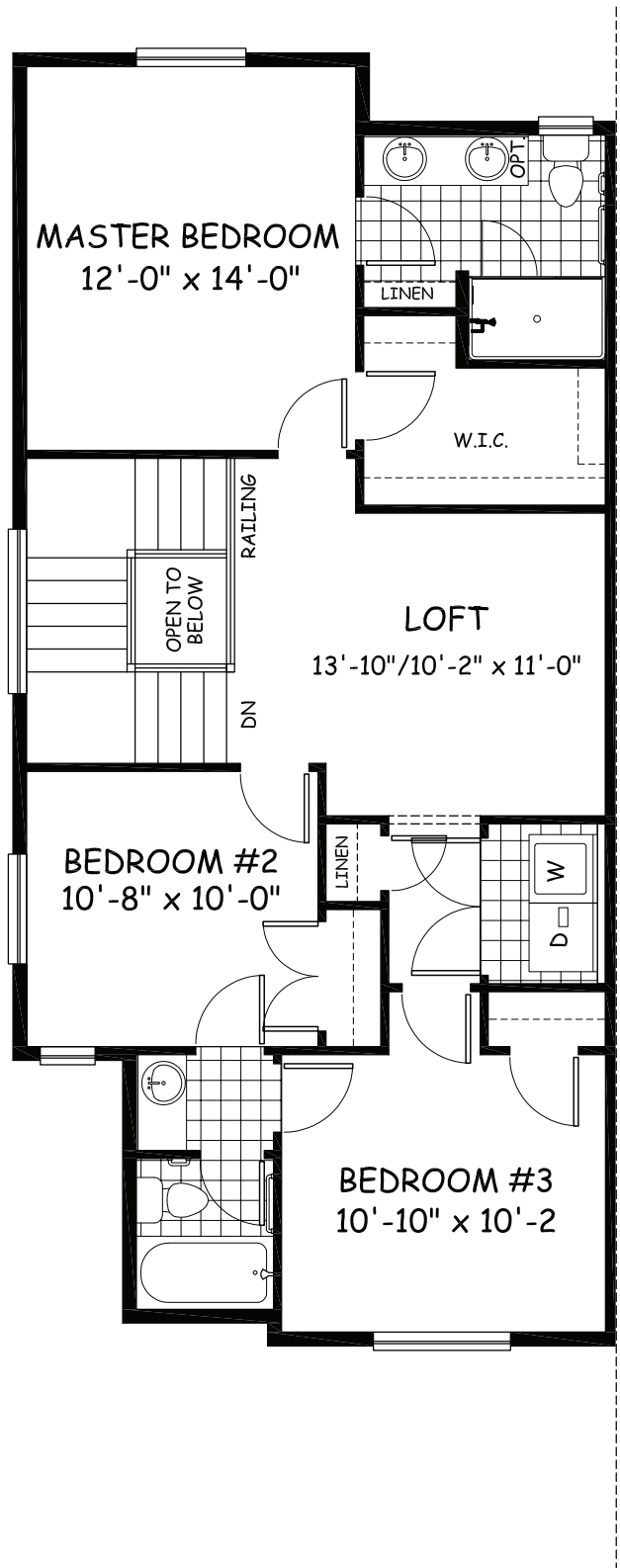
Upper Floor 888 sqft
