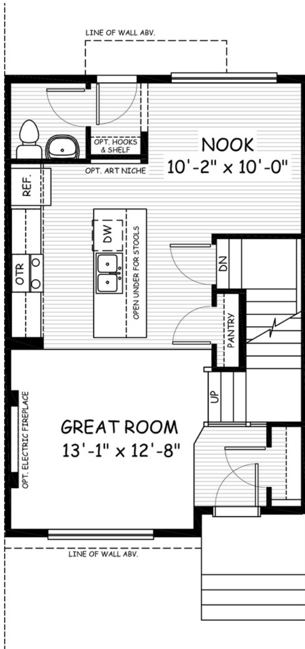
MAIN 600 sq.ft.
