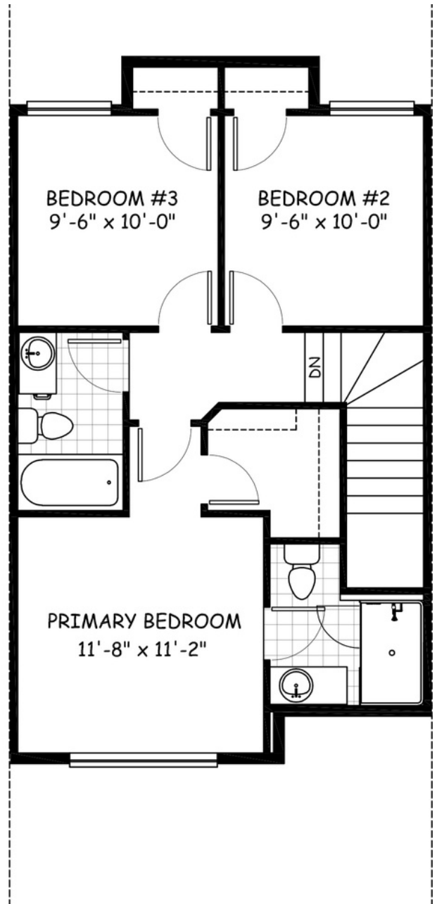
UPPER 580 sq.ft.
