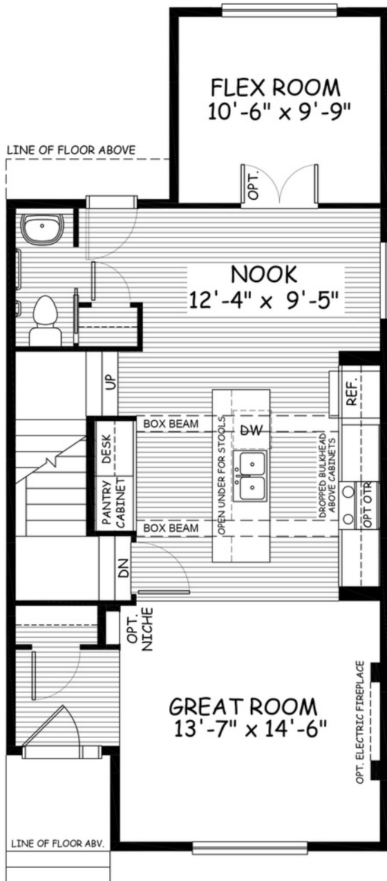
MAIN 768 sq.ft.
